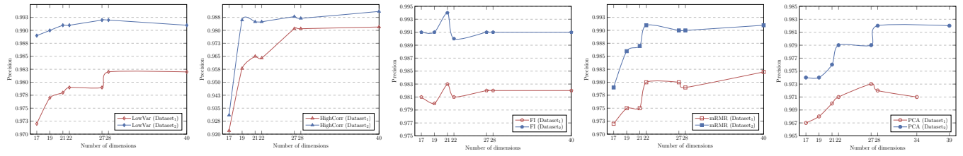
Fig. 5 The effect of increasing dimensions on the precision of the RF classification.
